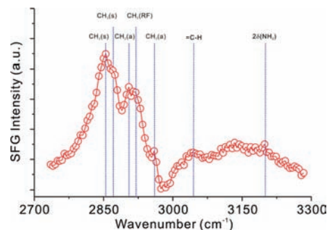
Figure 6. SFG vibrational spectra recorded during pyrrole hydrogenation (3 Torr pyrrole, 30 Torr H 2 ) over Pt (100) at 298 K. CH 2 (FR) represents Fermi resonance of the methyl group.
