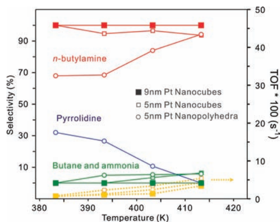
Figure 5. Pyrrole hydrogenation selectivity for Pt nanocrystals with different size and shape as a function of temperature. The color of the line coordinated to Scheme 2. “■”, “□”, and “○” represent 9 nm nanocubes, 5 nm nanocubes, and 5 nm nanopolyhedra, respectively. Feed was 4 Torr of pyrrole and 400 Torr of H 2 with a He balance.
