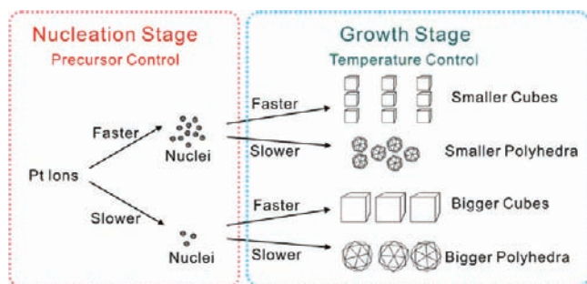
Scheme 1. Schematic Illustration of the Size and Shape Control of Sub-10 nm Pt Nanocrystals a
