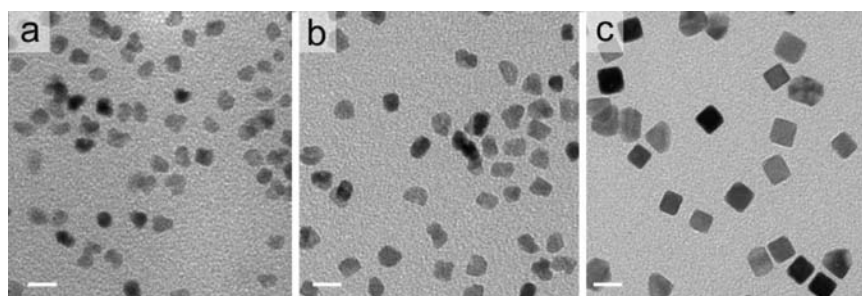
Figure 2. TEM images of 9 nm Pt nanocubes at different stages of the synthesis. (a) 2 min, (b) 5 min, and (c) 10 min. The scale bars are 10 nm in the TEM images.
