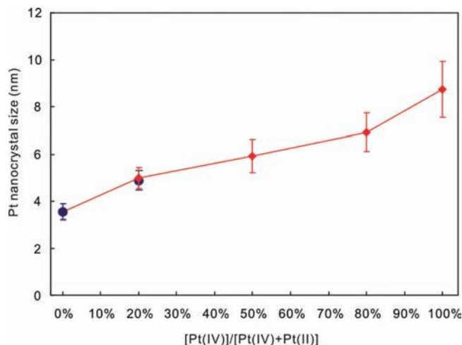
Figure 3. The size of Pt nanocrystals as a function of [Pt(IV) to Pt(IV) + Pt(II)] in the initial solution. The blue “●” represent nanopolyhedra, and the red “◆” represent nanocubes.
