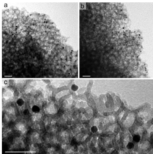
Figure 4. TEM images of Pt nanocrystals loaded onto mesoporous MCF-17: (a) 5 nm nanocubes, (b) 5 nm nanopolyhedra, and (c) 9 nm nanocubes. The scale bars are 100 nm in the TEM images.
