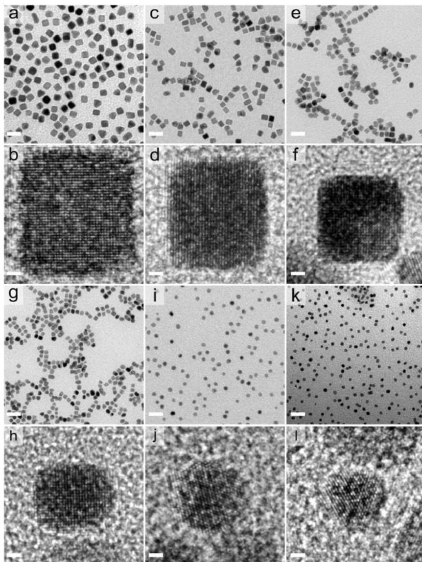
Figure 1. TEM and HRTEM images of Pt nanocrystals with different shape and size. TEM images of (a) 9 nm nanocubes, (c) 7 nm nanocubes, (e) 6 nm nanocubes, (g) 5 nm nanocubes, (i) 5 nm nanopolyhedra, and (k) 3.5 nm nuclei. HRTEM images of a single (b) 9 nm nanocube, (d) 7 nm nanocube, (f) 6 nm nanocube, and (h) 5 nm nanocube along the [100] zone axis. HRTEM images of a single (j) 5 nm nanopolyhedron, and (l) 3.5 nm nucleus along the [111] zone axis. The scale bars are 20 nm in the TEM images and 1 nm in the HRTEM images.
